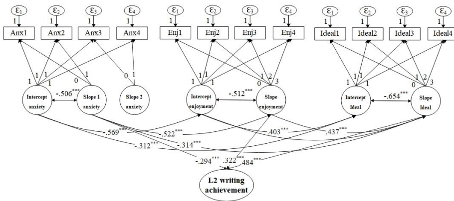
Figure 1. Conditional LGCM
